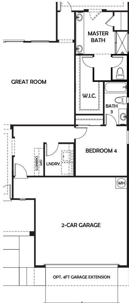
OPT. BEDROOM 4 / BATH 3 I.L.O. 3-CAR TANDEM GARAGE
